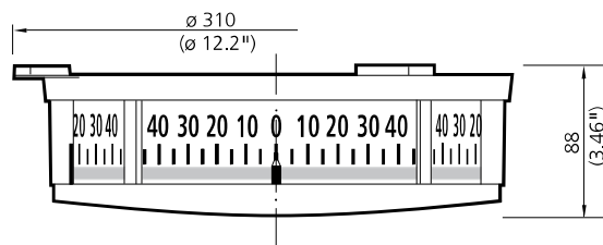
Three-face rudder angle indicator
