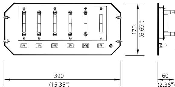
Distribution plate
